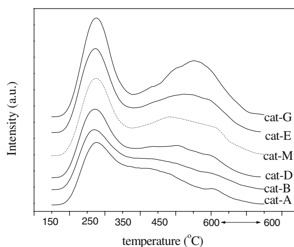
Figure 4. NH 3 – TPD curves of samples.
